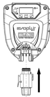
Figure 4: Power supply connector connection
