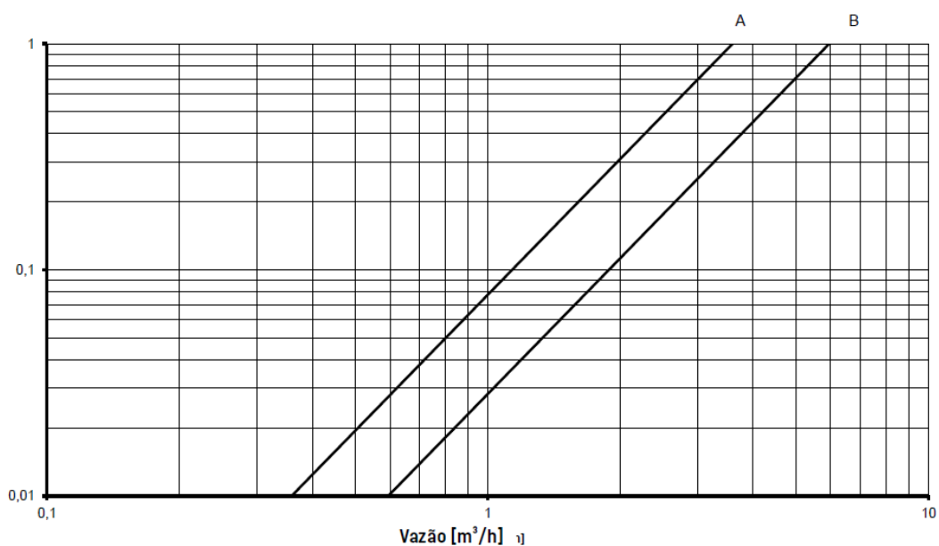
Pressure loss diagram Δp
