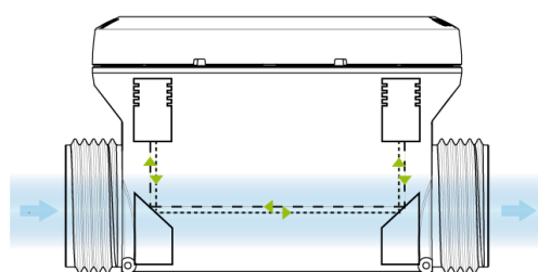
Principle of ultrasound signal path
