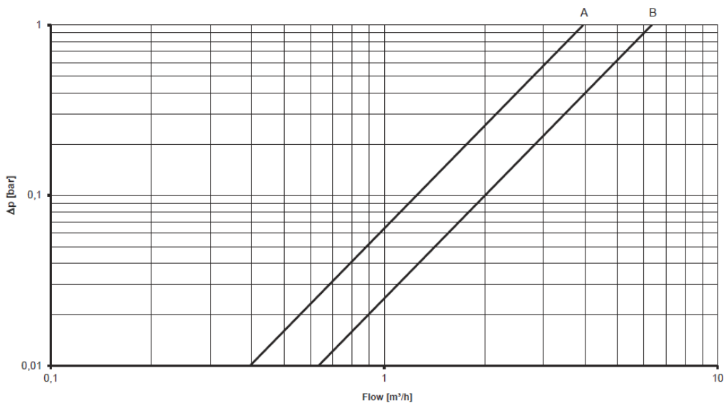
Pressure loss diagram Δp
